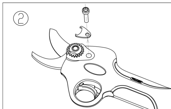
2. Remove adjustment clip bolt and adjustment clip.
