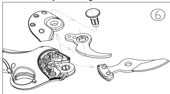
6. Remove cover and disassemble blade set.
