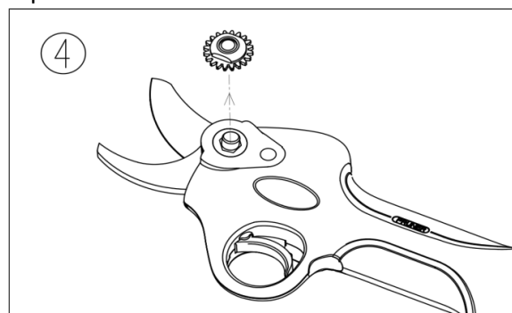
4. Remove adjustment gear nut.
