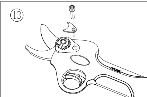
13. Secure gear nut with clip and insert bolt.
