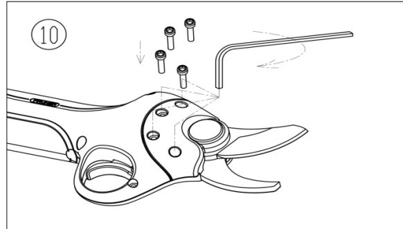
10. Tighten 4 cover screws with allen wrench.
